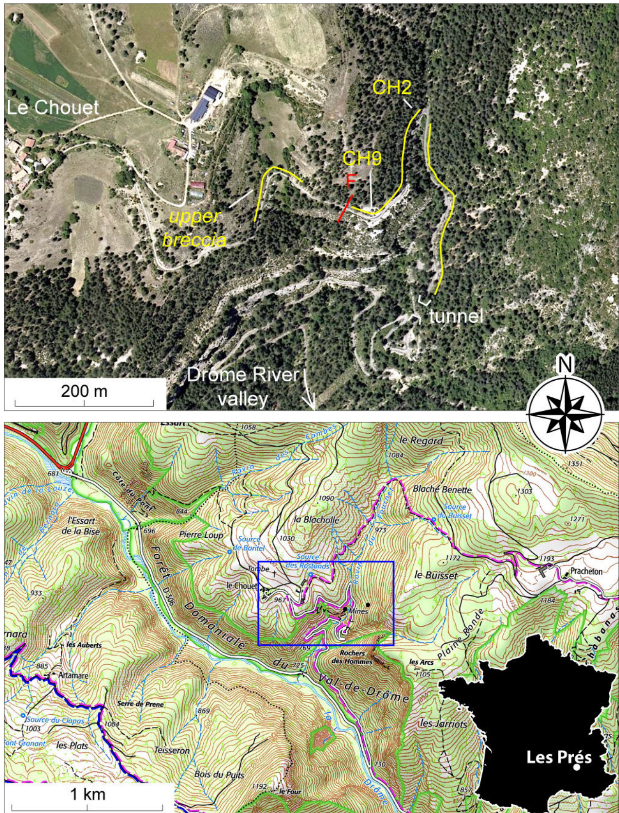
Figure 1: Topographic map of the Le Chouet area (A) and location of the sections studied (B).
